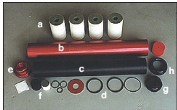
Fig. 3-1 Many parts go into a solid rocket motor
