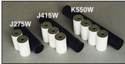
Fig. 3-7 Similar propellant slugs can be 'stacked' in order to increase the average and total impulse
