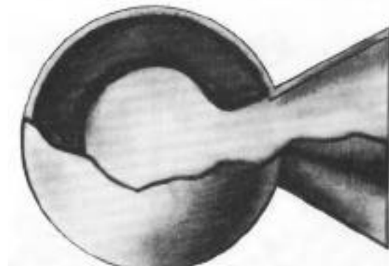
Solid fuel rocket motor with a high mass fraction.
